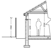
Proposed Cross Section.
